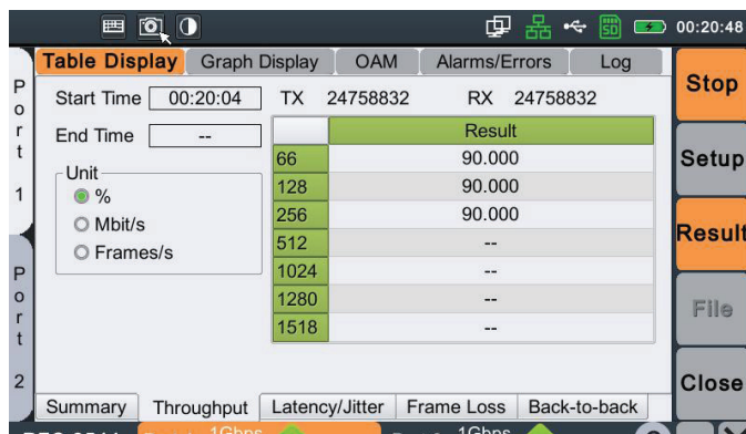
RFC 2544 throughput measurement results
