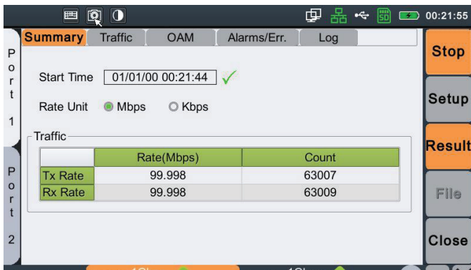
Ethernet Loopback measurement screen
