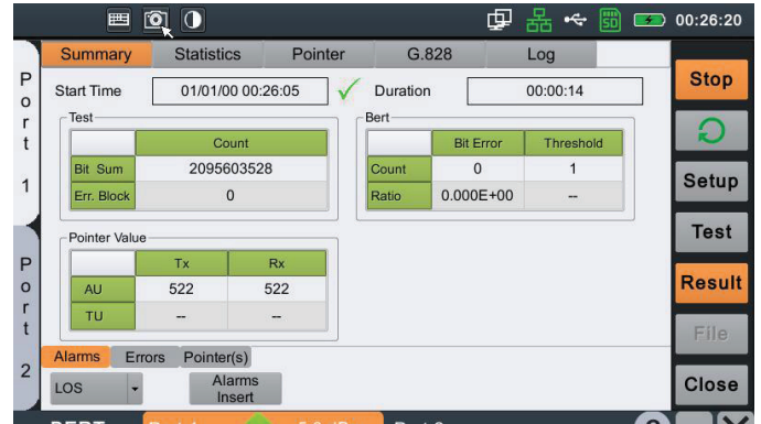
SDH Bert measurement screen
