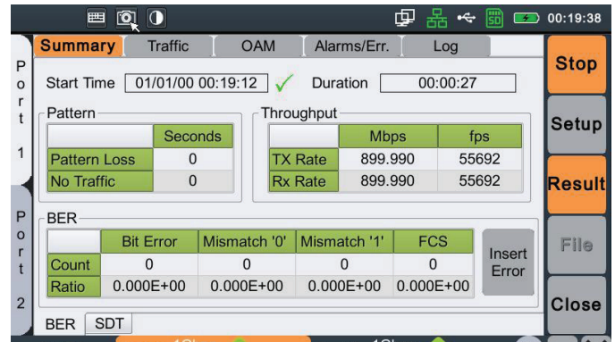
Ethernet BERT results. Click "Insert" to insert a specified number of bit/FCS errors.
