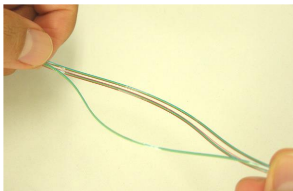
Sub-group of 4-fiber is extracted from 12-fiber ribbon.
