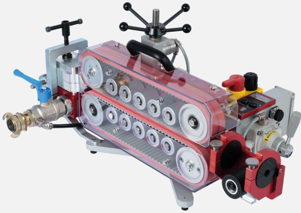
V3 FIBER BLOWING MACHINE
