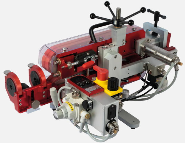
V3 FIBER BLOWING MACHINE
