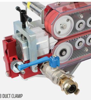
V3 DUCT CLAMP
