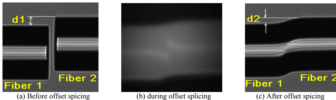
Figure 2. Offset splicing method for arc power calibration. The offset variation is measured at fiber axis by d1-d2 . The Fiber 1 and Fiber 2 are of the same fiber type. This method works well for telecom fibers with 125 micron diameter only.
