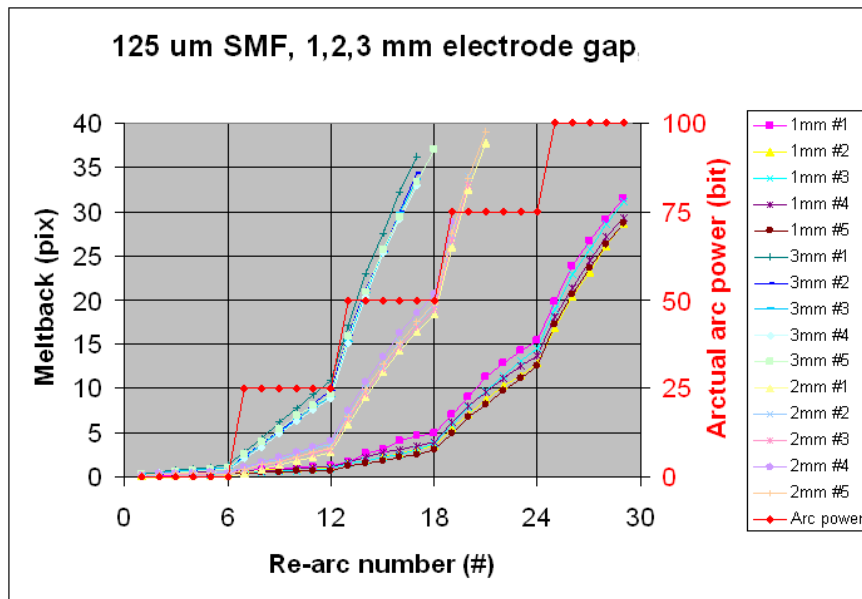
Figure 4. Meltback test with different arc power levels and different plasma zones. The arc power varies from 0 bit (~ 10.5 mA) to 100 bit (~ 14.5 mA) with 25 bit increments. The plasma zone varies from a 1 mm electrode gap to a 3 mm electrode gap with 1 mm increments. Each curve represents one meltback test which consists of 20 to 30 re-arcs of 0.3 sec arc length. 5 tests were performed for each plasma zone setting to verify the consistency. The red curve is showing the arc power. Each dot on the curve represents one re-arc.
