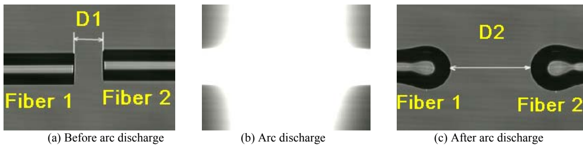
Figure 1. Traditional meltback method for arc power calibration. The meltback value is measured at fiber axis by subtracting D1 from D2. Fiber meltback causes heavy silica particles to deposit on the electrode tips for LDF fiber types, and leads to inaccurate arc calibrations.
