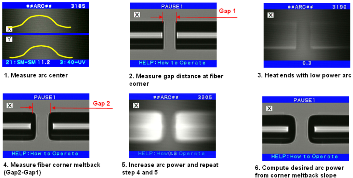
Figure 3. Process illustration for viable arc power meltback method used in arc power calibration. The axis meltback is very limited and not measurable in many cases. The electrode condition is not impacted by this arc calibration
