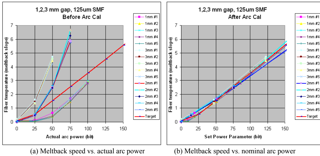
Figure 5. Meltback speed computed from the tests shown in Fig. 4 is projected from the actual arc power domain to the nominal arc power domain by the arc calibration process. After arc calibration, the same power setting will achieve the same fiber temperature (meltback speed) regardless of the plasma zone settings. The Y axis indicates the scale of pixels per pre-arc
