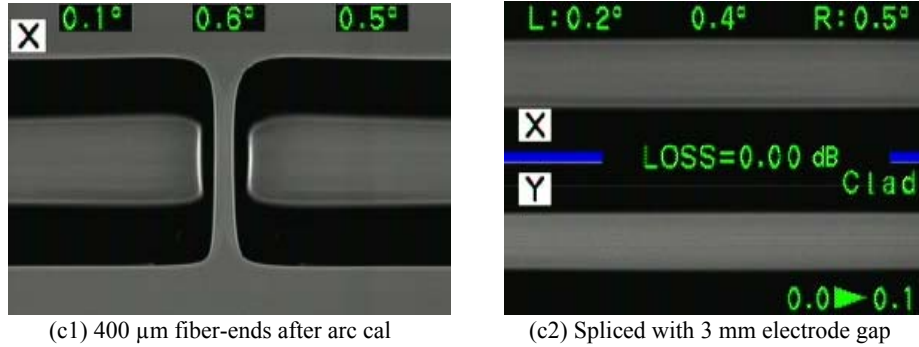
Figure 6. Fiber-ends after arc calibration and splicing for 125, 220, and 400 micron glass diameter fibers shown in groups (a), (b), and (c), respectively. The fibers are also spliced with different plasma zone settings. The same nominal power setting is used for all above fibers and plasma zones, to get similar splice results. In group (c) there is no picture for 1 mm electrode gap, since the small plasma zone is not strong enough to splice 400 micron fibers.
